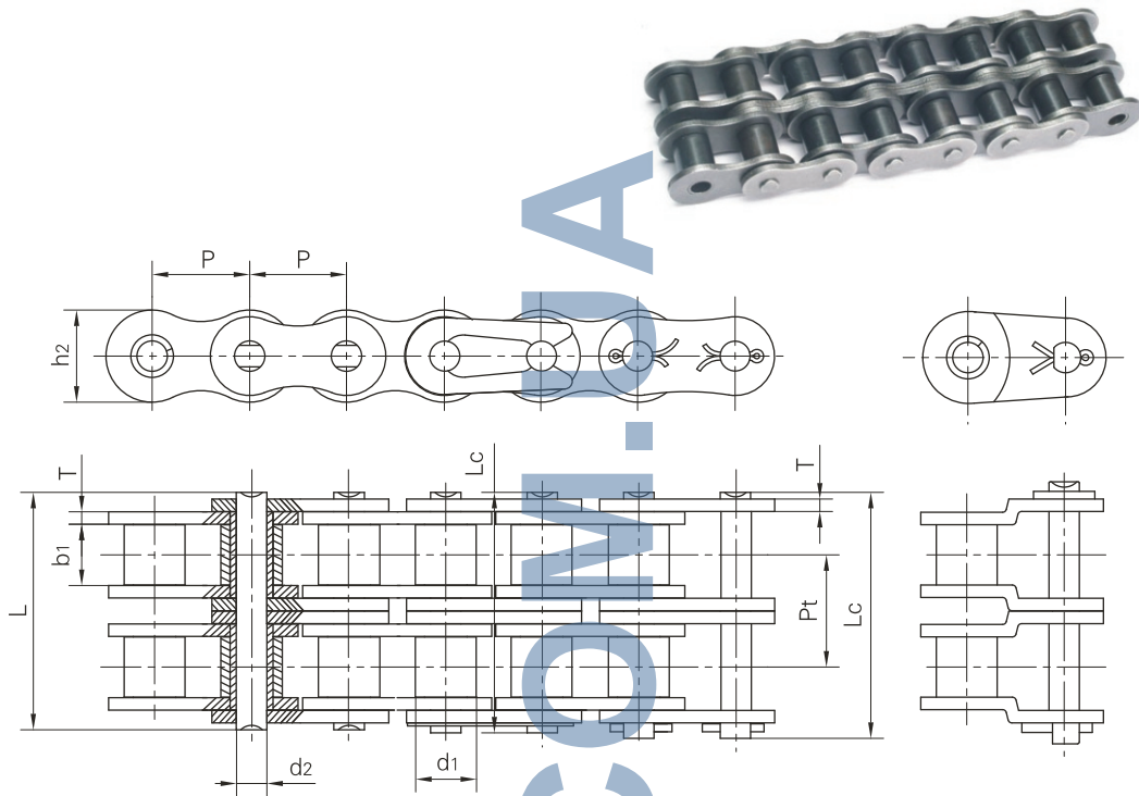
双排滚子链/套筒链 Duplex roller chains & bushing chains
